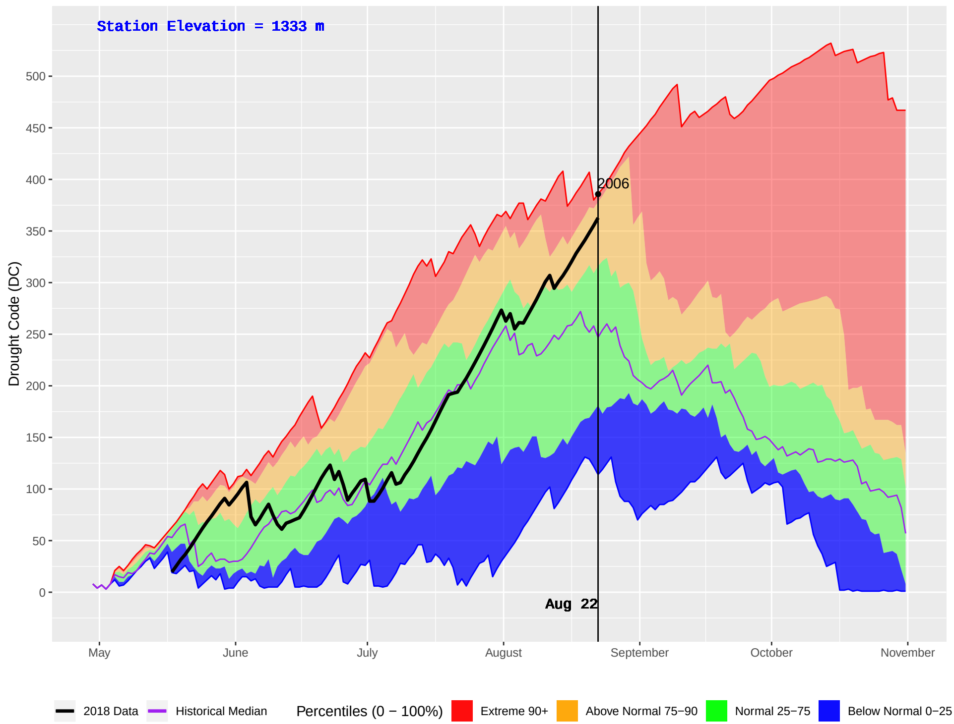
GOLDSTREAM 2 (919) : Historical (2005–2016) and Current (2018) Daily Drought Code (DC)
