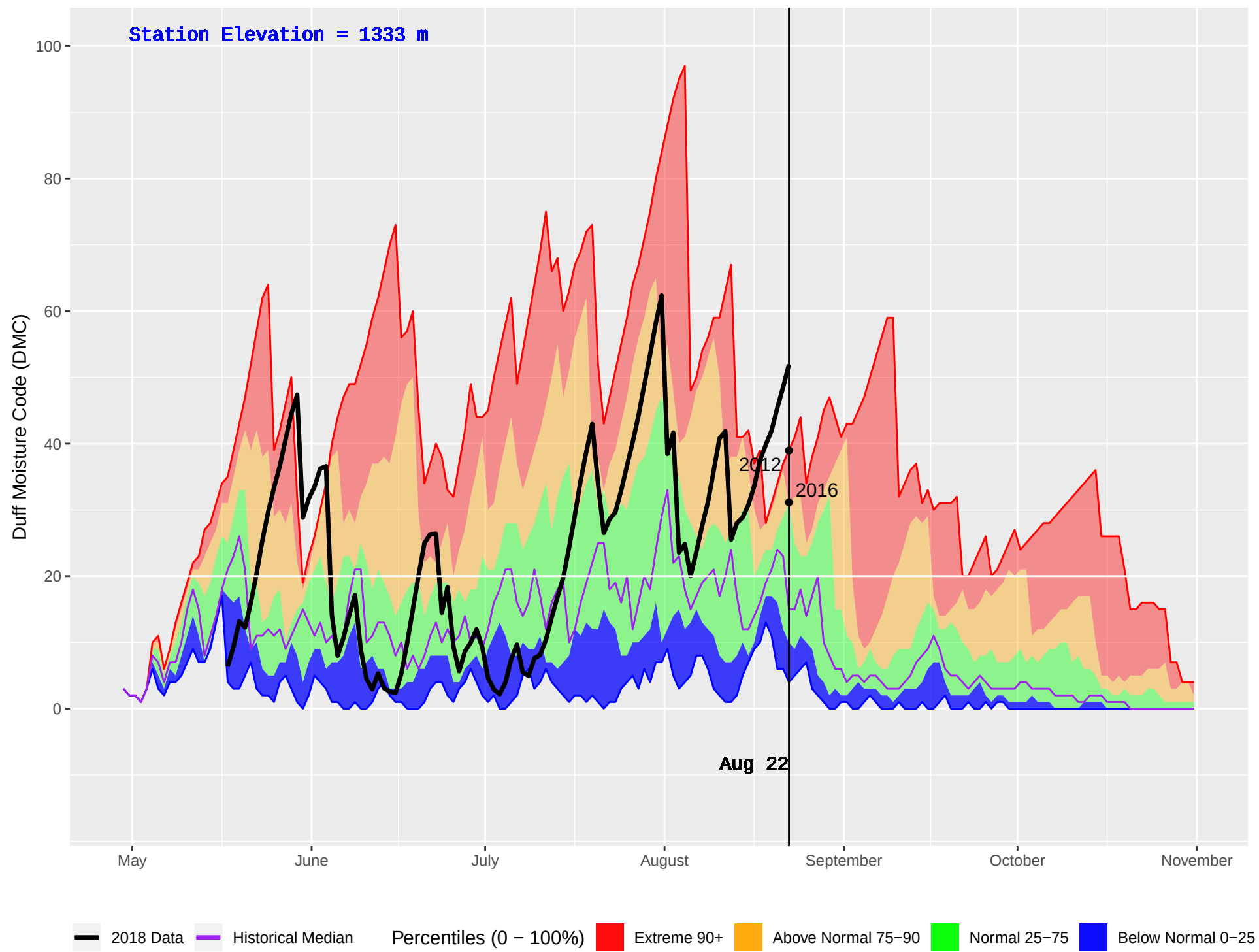
GOLDSTREAM 2 (919) : Historical (2005–2016) and Current (2018) Daily Duff Moisture Code (DMC)
