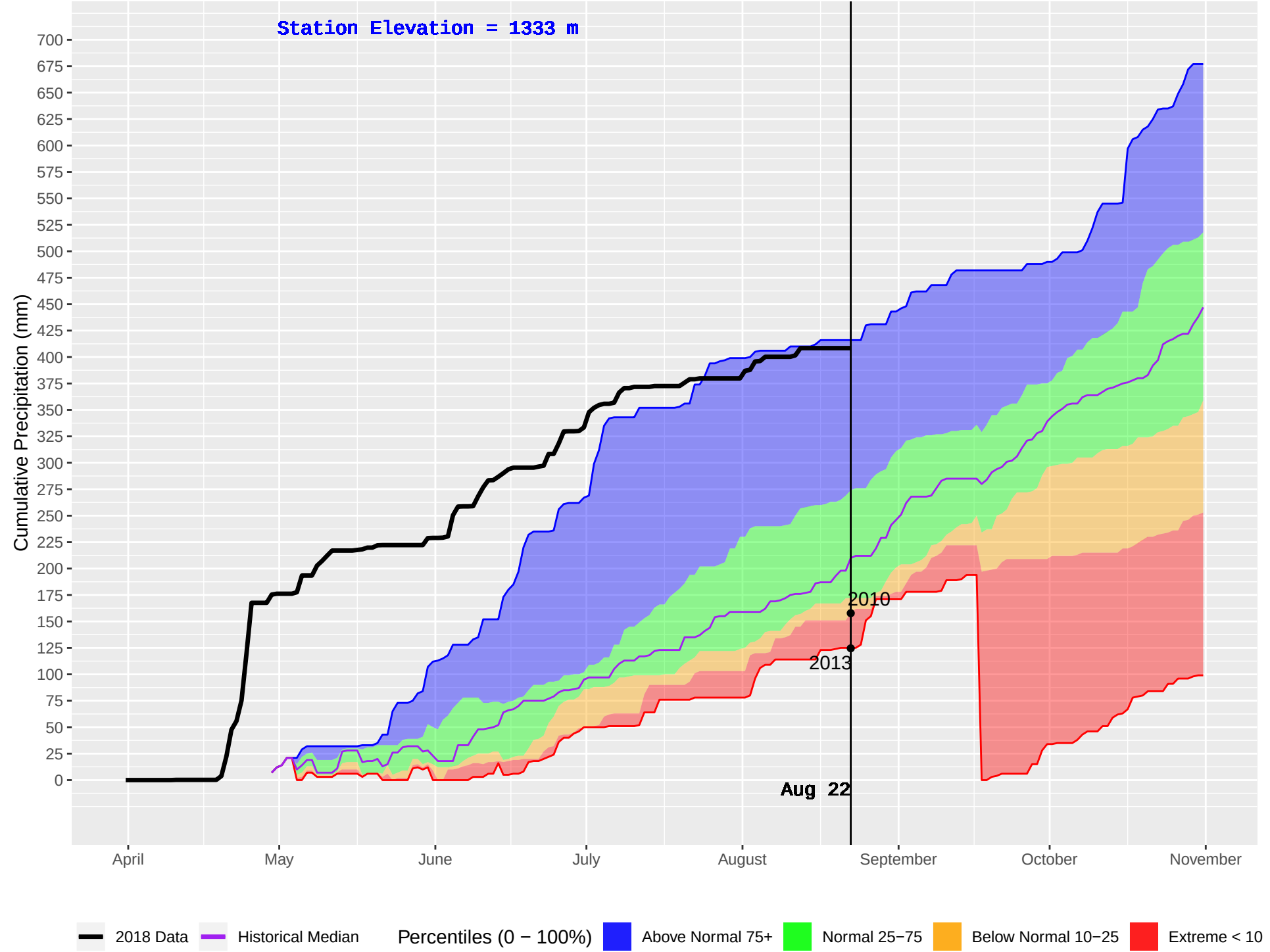
GOLDSTREAM 2 (919) : Historical (2005–2016) and Current (2018) Daily Cumulative Precipitation
